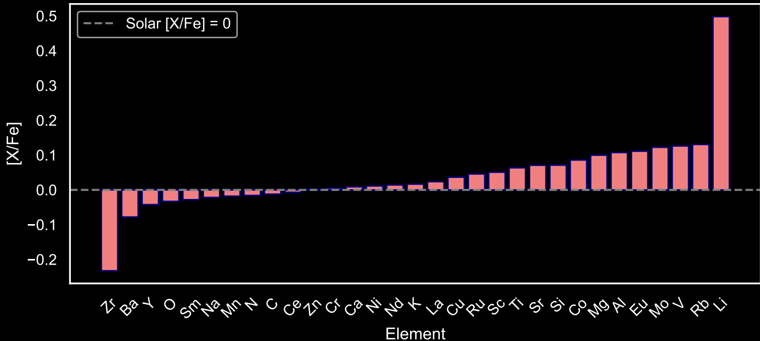
Abundance Pattern for GALAH Main Sequence Stars: Star Field [15] (N=141)
