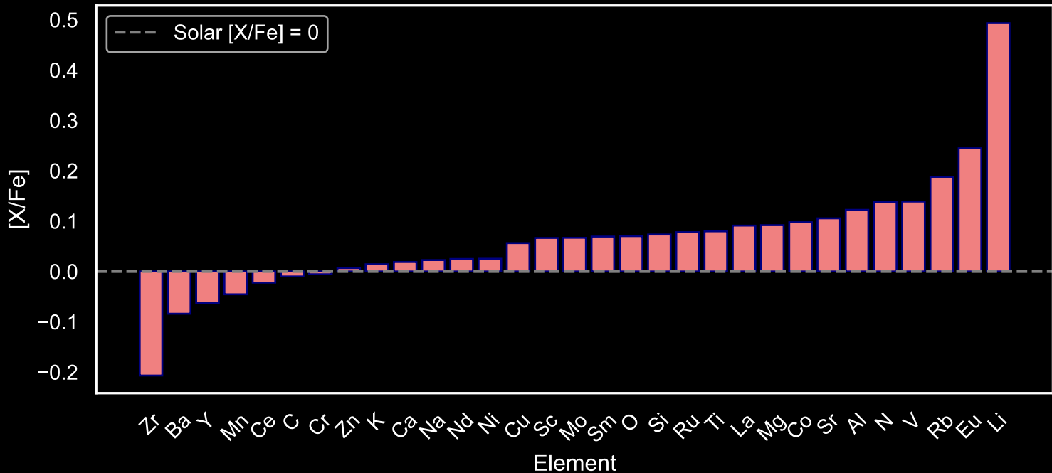
Abundance Pattern for GALAH Star Field [15] (N=284)
