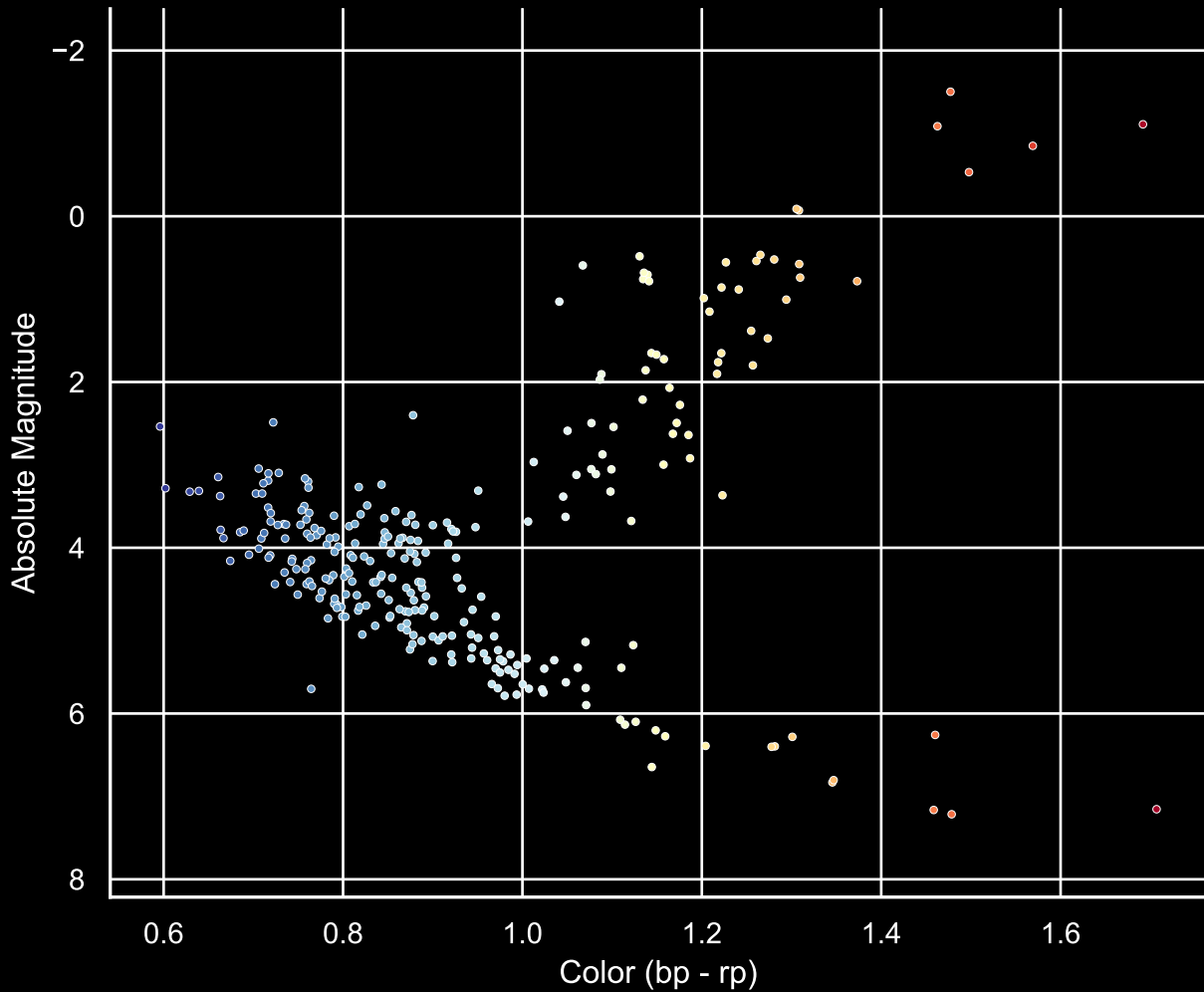
GALAH Hertzprung-Russel Diagram Field [15] Ra [328.04] Dec [-55.84]
