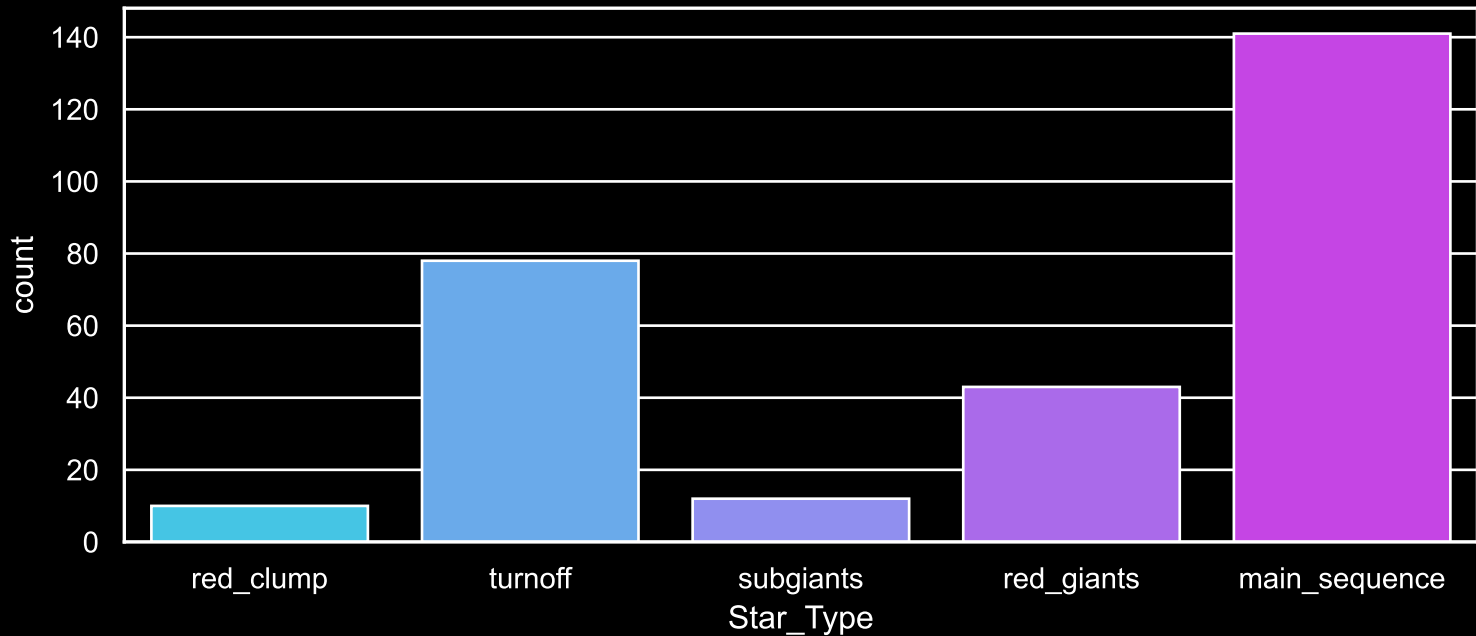
Field [15] Count plot of Star Type
