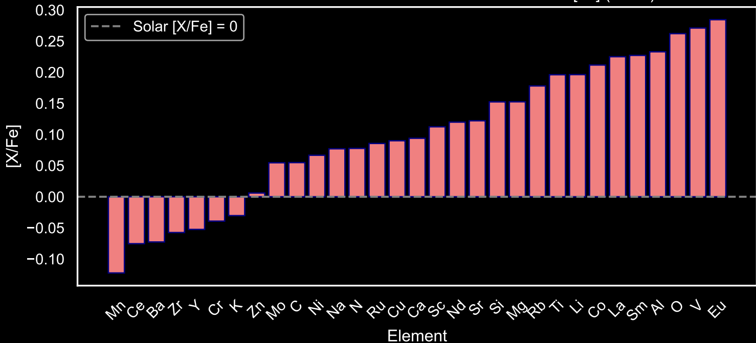
Abundance Pattern for GALAH Red Giants: Star Field [15] (N=53)
